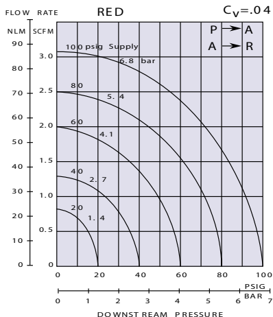
0.062 in (1.6) Orifice
