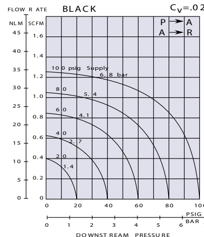
0.031 in (0.8) Orifice
