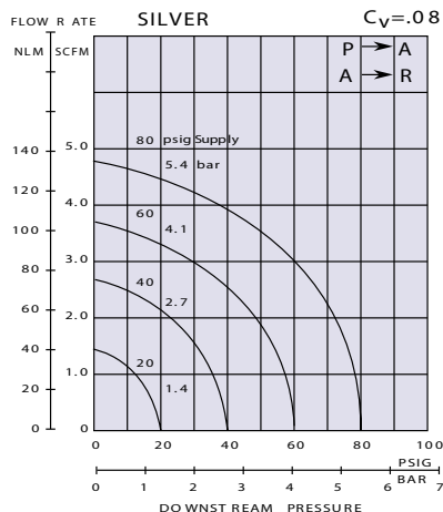
0.089 in (2.3) Orifice
