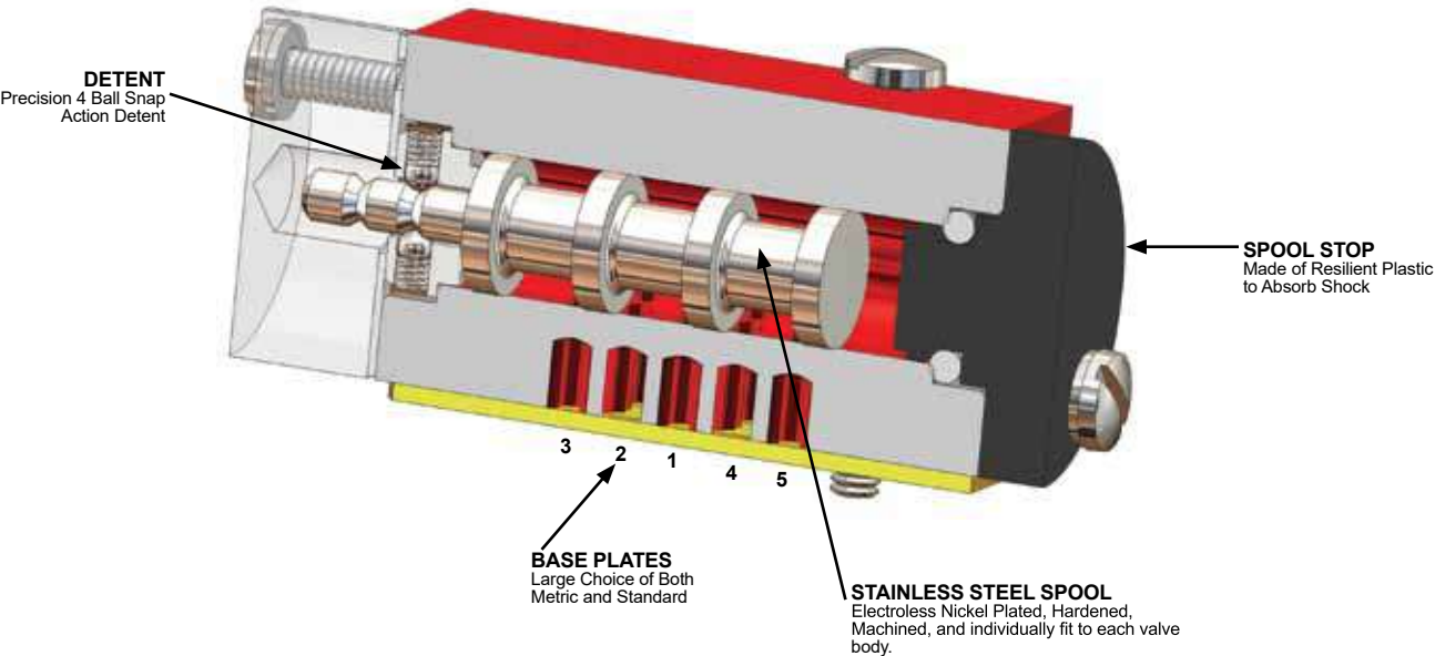
DOUBLE AIR PILOT - DETENTED
